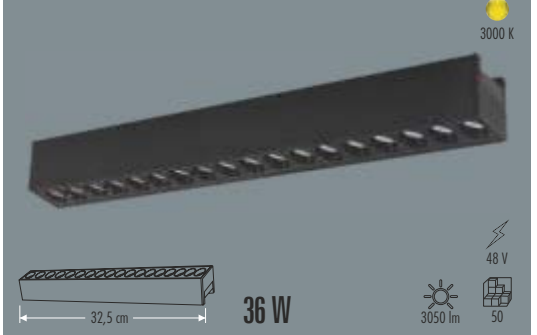
KN-05059 MAGNETIC
