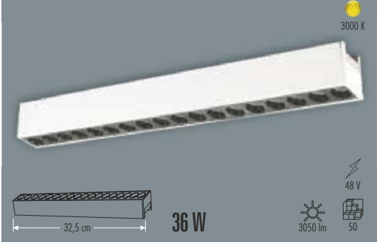
KN-05076 MAGNETIC
