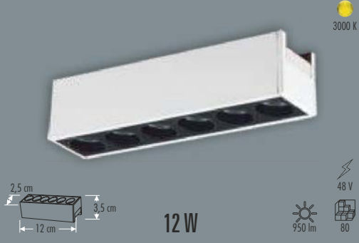
KN-05077 MAGNETIC
