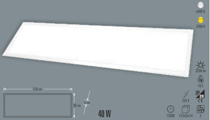
KN-43363 30 x 120 FLAT PANEL LIGHT
