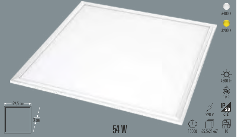
KN-42483 60 x 60 FLAT PANEL LIGHT
